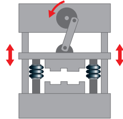
Pneumatic ram weight compensation
