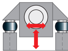
Washing machines
