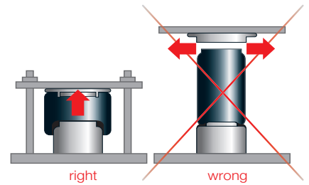
Up stop
