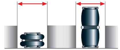
Installation space
