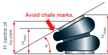
Tilt angle
