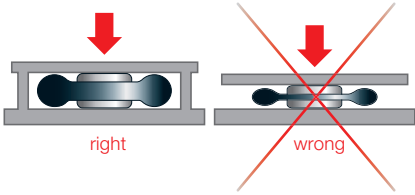
Down stop
