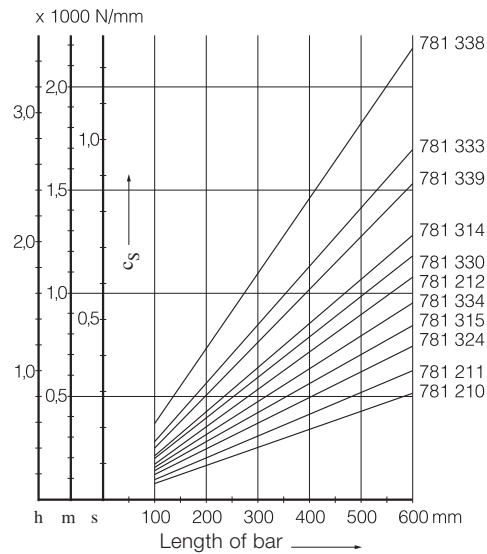
Spring rate for compression stress c_S
