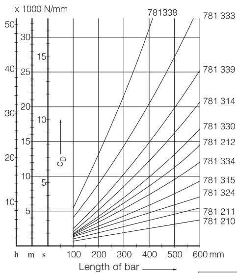
Spring rate for compression stress c_D
