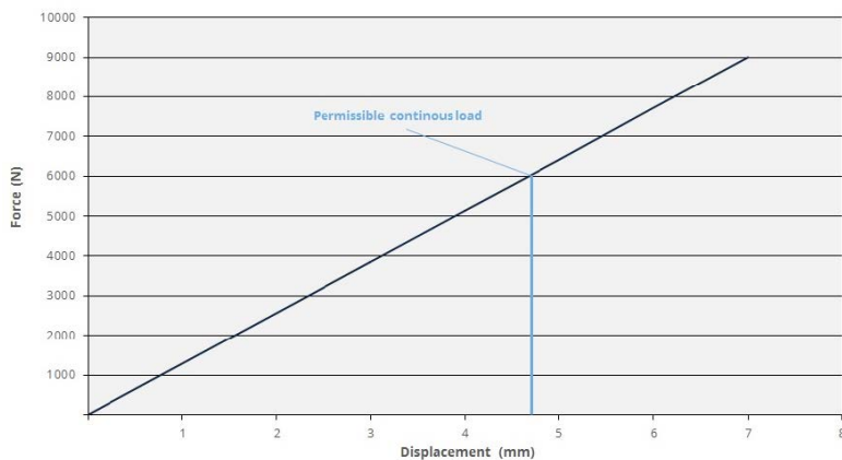
Force-deflection curve in Z direction
